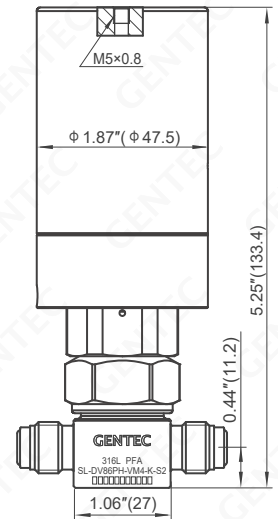
Pneumatic (3500 psi)
