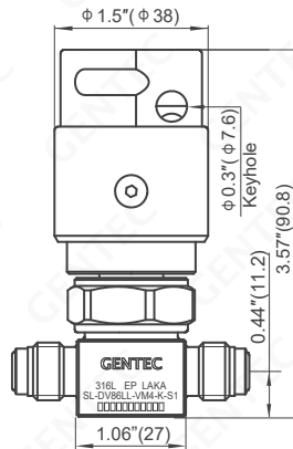
LOTO Handle (300 psi)
