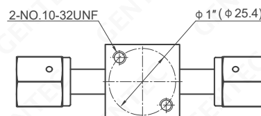
Rear Bracket Mounting
